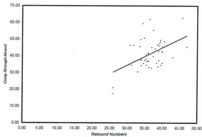
Fig. 6 – Calibration Graph
